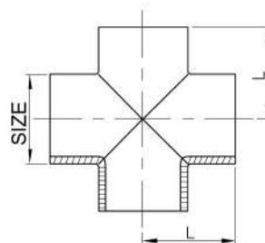
WELDED CROSS SHORT 9WWW
