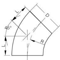
WELDED ELBOW 45° 2KSX
