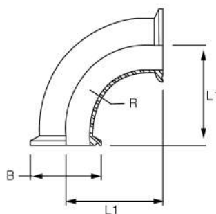
CLAMPED ELBOW 90° 2CMP
