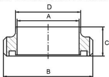
SMS Threaded Male Ferrule
