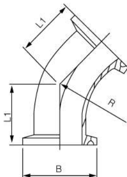
CLAMPED ELBOW 45° 2KMP
