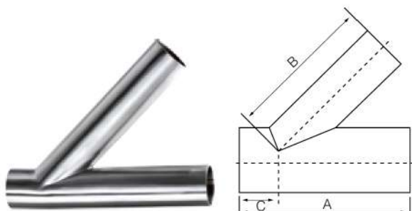
WELDED TEE Y LATERAL 28WA
