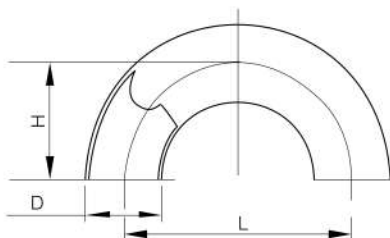
WELDED ELBOW 180° 2WU
