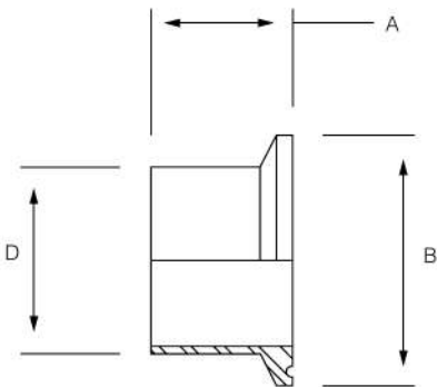
LONG FERRULE C14AM7
