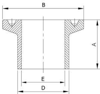
SHORT FERRULE HEAVY DUTY C14-H
