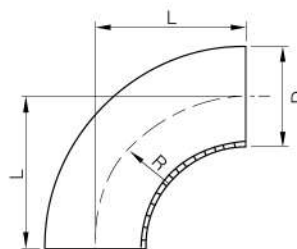
WELDED ELBOW 90° 2SX
